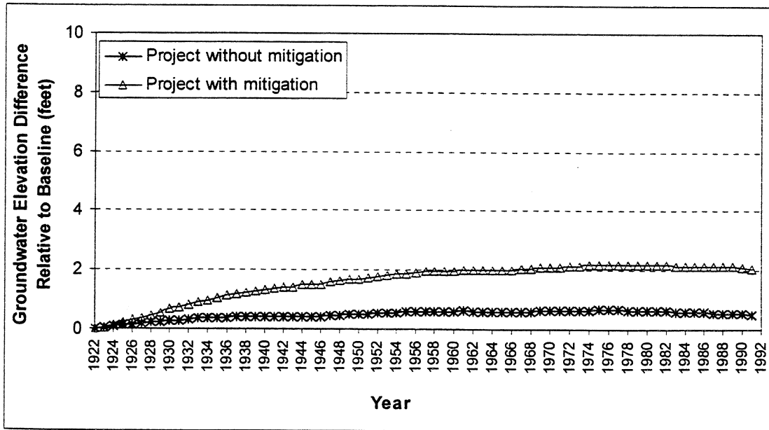
Figure A.32 Groundwater Elevation Difference Relative to “Baseline Condition” for Aquifer 2 Underlying McClellan Contaminant Plumes (Node #36)
